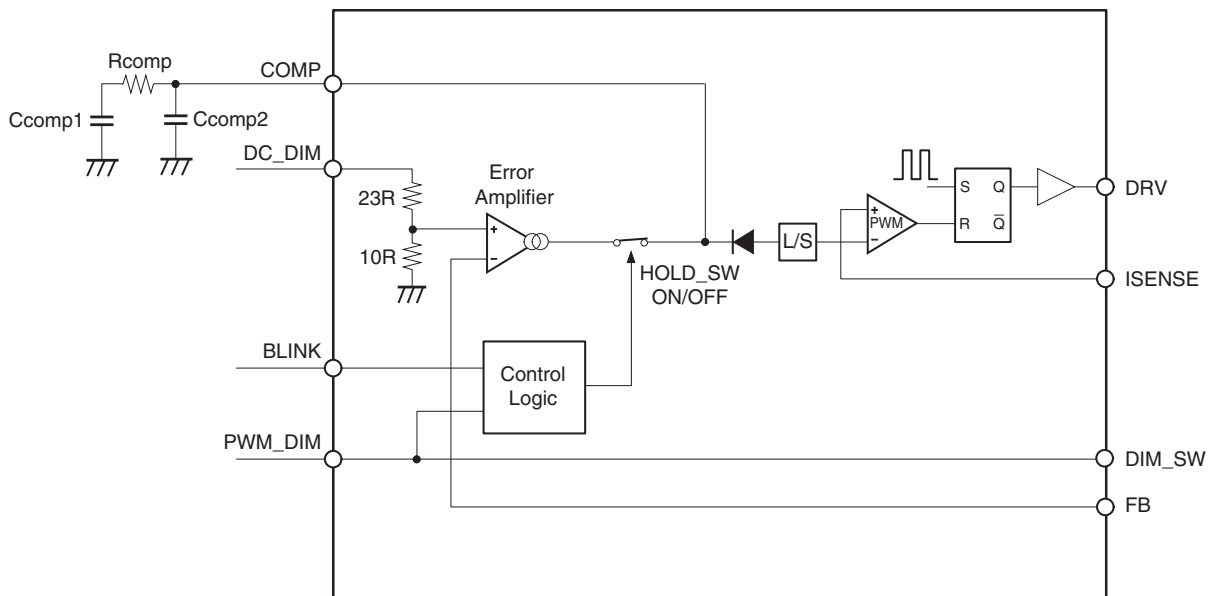
Fig. 13. COMP Pin Peripheral Equivalent Circuit
