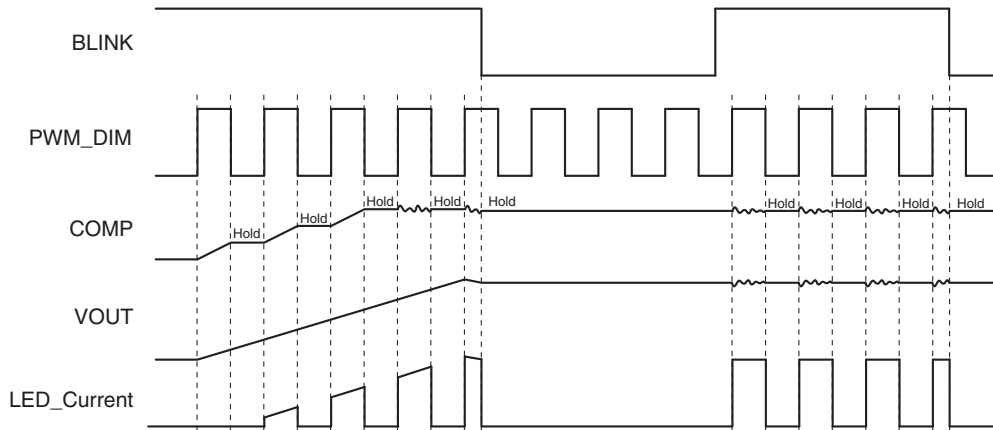
Fig. 12. COMP Pin Hold Function Timing Chart
