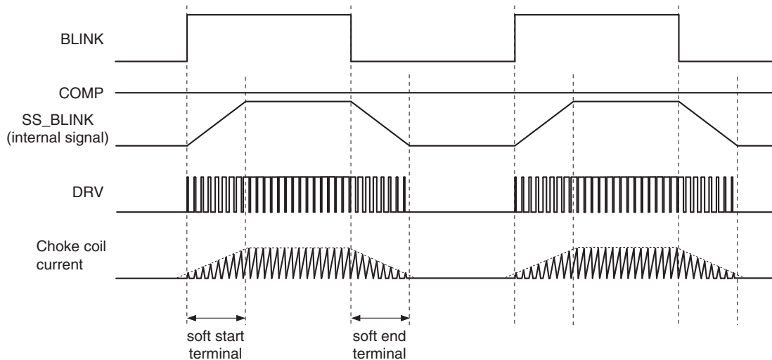
Fig. 11. Overview of DC-DC Converter Operation During Blinking
