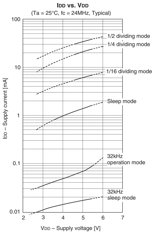
Fig. 13. Characteristic curves
