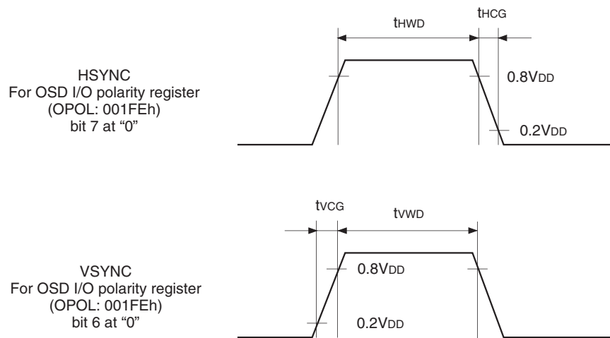
Fig. 10. OSD timing
