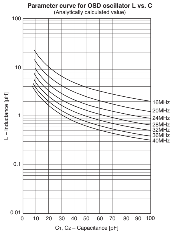
Fig. 13. Characteristic curves
