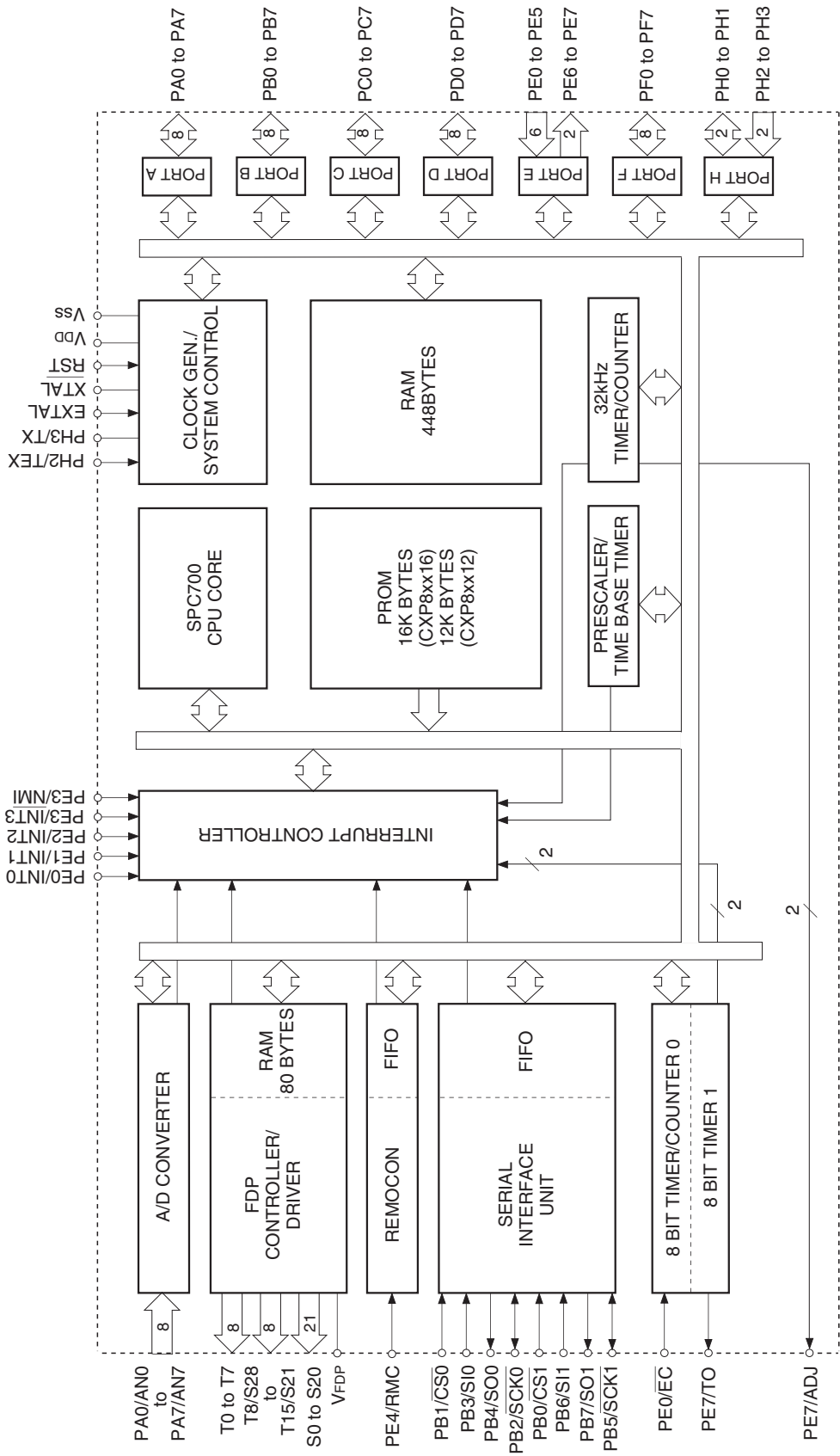
Block Diagram
