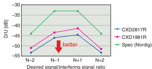
TASK_3_23 Immunity to "Analog" Signals in Other Channels 666 MHz 64QAM CR = 3/4 GI = 1/4
